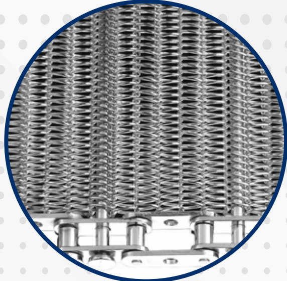
Chain Drive
